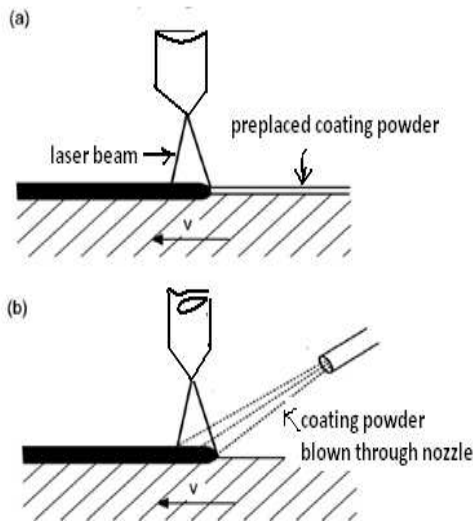
Fig.1: Laser coating by (a) Preplaced powder method and (b) Blown powder method [Ref-H. Gedda 2004 [7]]
