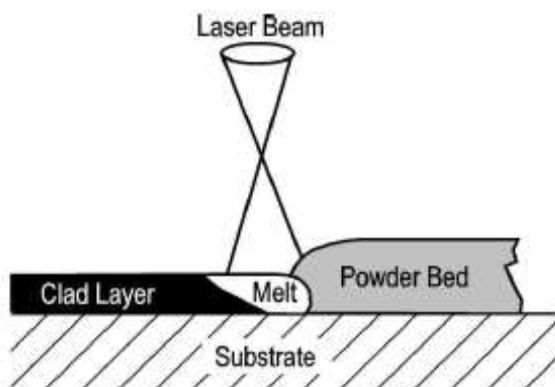
Fig. 2: The preplaced powder cladding technique
